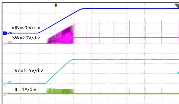
Figure 10-10. Start-Up with VIN rising I_{OUT}=0A
