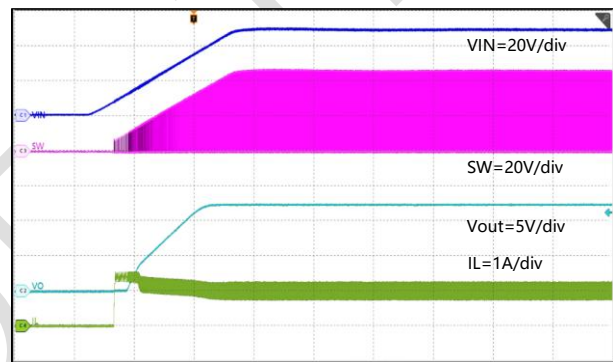
Figure 10-11. Start-Up with VIN Rising I_{OUT}=1A
