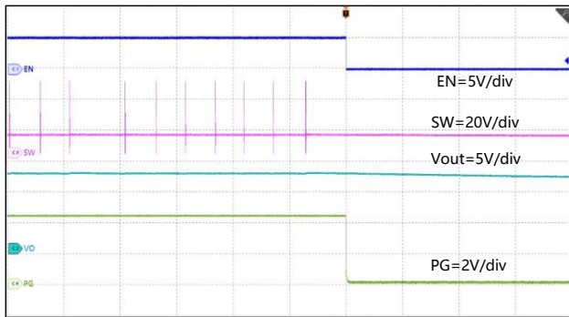
Figure 10-8. Shut-down with EN, I_{OUT}=0A
