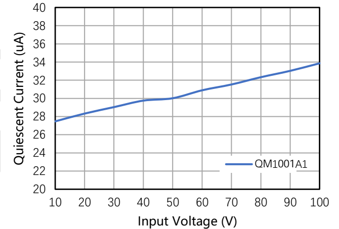
Figure 7-10. IQ Current vs Input Voltage
