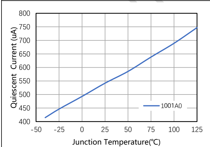
Figure 7-11. IQ Current vs Junction Temperature
