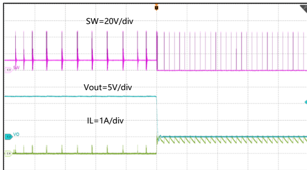
Figure 10-16. Normal Operation to Hard-short
