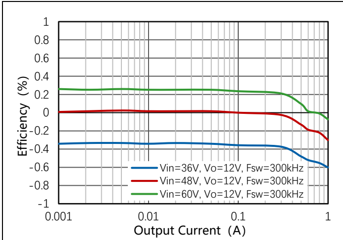
Figure 7-7. Load Regulation QM1001A0
