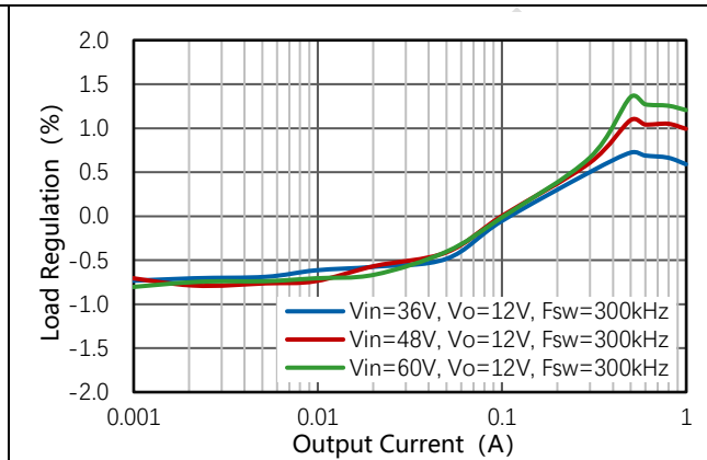
Figure 10-3. V_{OUT} Vs. Load Regulation
