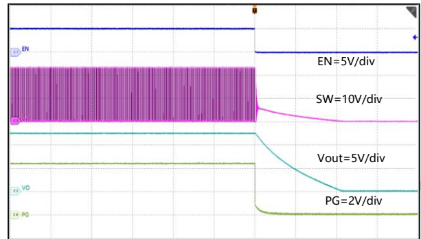
Figure 10-9. Shut-down with EN, I_{OUT}=1A
