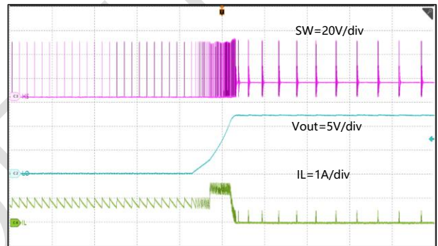
Figure 10-17. Hard-short Recover
