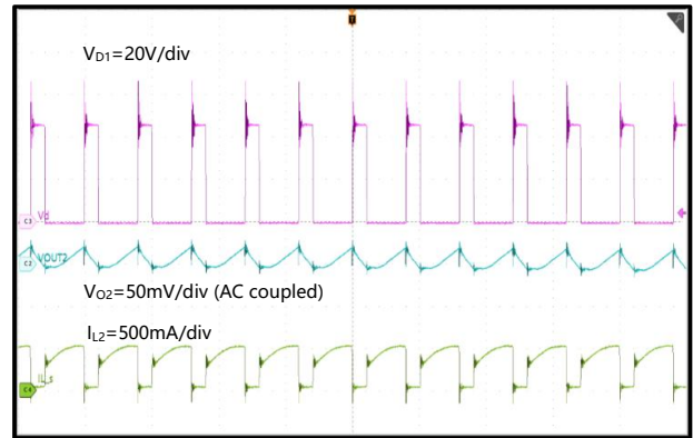
Figure 10-24. Steady State in Secondary Side, I_{OUT1}=0.3A , I_{OUT2}=0.3A
