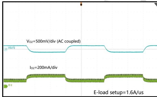
Figure 10-25, Load Transient in Secondary Side I_{OUT1}=0A , I_{OUT2}=0.1A-0.2A
