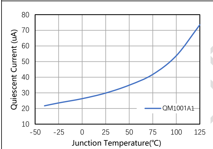
Figure 7-9. IQ Current vs Junction Temperature
